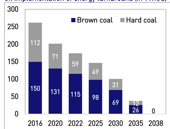
Figure 2: Coal-fired electricity production up to 2035 on implementation of energy turnaround (in TWh/a)
